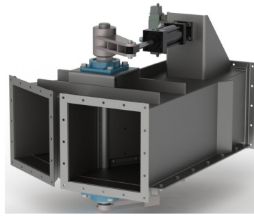
DIVERTER VALVES
