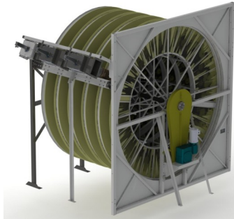
CIRCLE-VEE FILTERS
